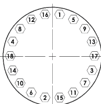
18 BOULONS 18 BOLTS
