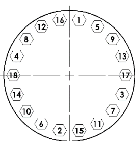
18 BOULONS 18 BOLTS
